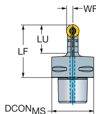
C x -SRDCN..HPA
