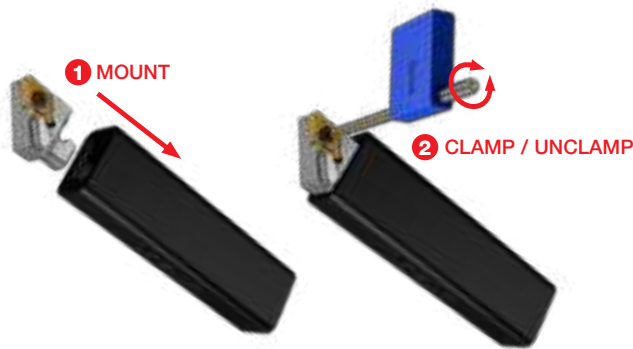
Auxiliary Handle for Easy Insert Indexing NQCH Head
