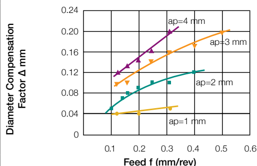
Insert: GIP 3.00E-0.4 Toolholder: GHDR 25-3
