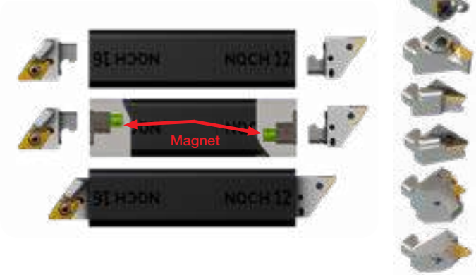
Double-Sided Handle, for Both 12 and 16 Head Sizes
