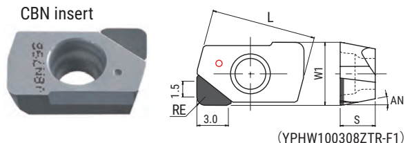
CBN insert
