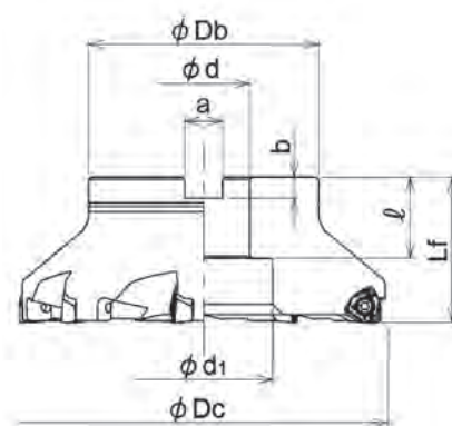
Fig.2 (No coolant hole)
