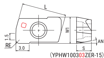
"Mirror Insert" for finishing side & bottom face (YPHW1003 * * ZER-15) (YPHW100308ZTR-F1) (YPHW100308ZER-F)
