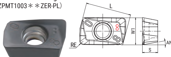
Shoulder insert for Ti alloy (ZPMT1003 * * ZER-SL)
