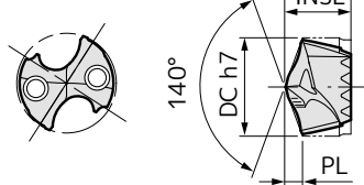
Indexable Head MTL type Diameter ø17.4 to 22.7mm
