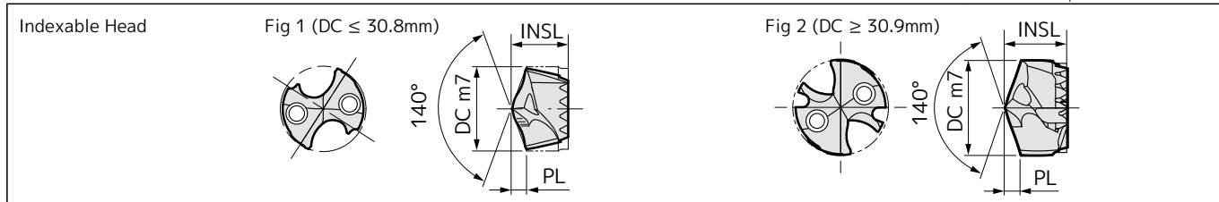
Indexable Head MTL type Diameter ø22.8 to 28.1mm
