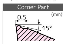
Chipbreaker Cross Section (CCGT09T300 type)
