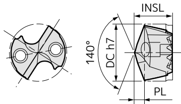
Indexable Head MSL type Diameter \varnothing 17.4 to 22.7mm
