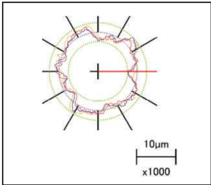
Circularity: 4-flute Regular-pitched
