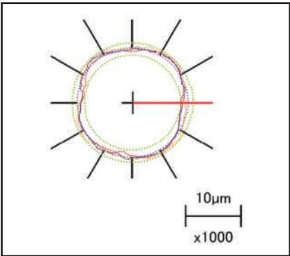
Circularity: 4-flute Irregular-pitched
