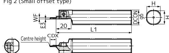
Fig 2 (Small offset type)
