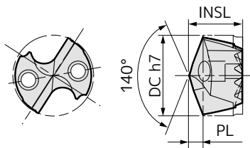
Indexable Head MSL type Diameter \varnothing 28.2 to 30.8mm
