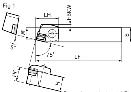
Figure shows right-handed (R) tool.
