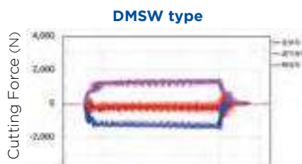
No Chattering
