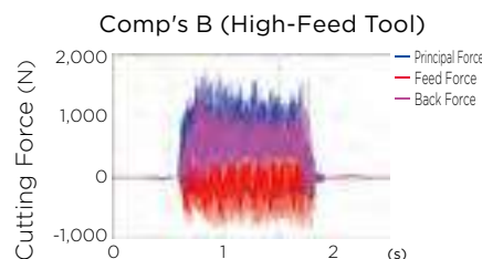
Heavy Chattering
