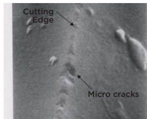
Cutting edge with microscopic irregularities
