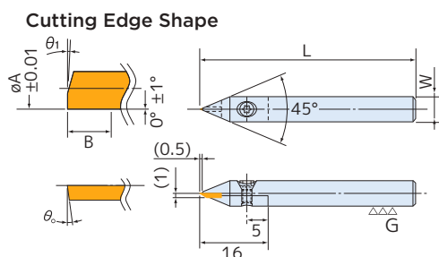
Cutting Edge Shape
