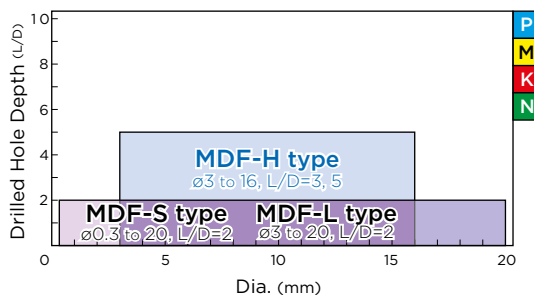
Flat MULTIDRILL MDF series
