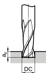
Slot Milling
