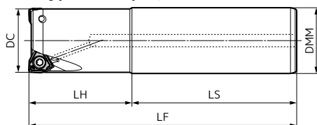
(Shank type Example)
