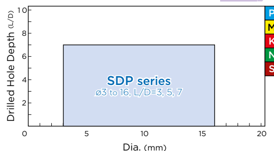
General-purpose SumiDrill Power SDP-type
