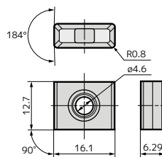
Fig 1 (General-purpose G type)
