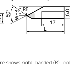
Fig 2 (Threading)
