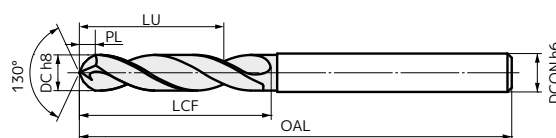
Fig 2 (Diameter ø4.851 to 10.0mm)
