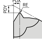
Close-up of Cutting Edge
