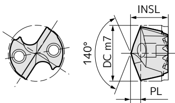
Indexable Head MSL type Diameter ø28.2 to 30.8mm
