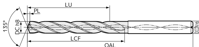
Fig 2 (Diameter ø2.5 to 20.0mm, double margin)
