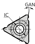
Chipbreaker Insert for Square Grooves BF type (Coated Carbide) Dimensions (mm)
