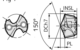
Indexable Head MB type Diameter \phi 24.5/24.7\text{mm} Dimensions (mm)
