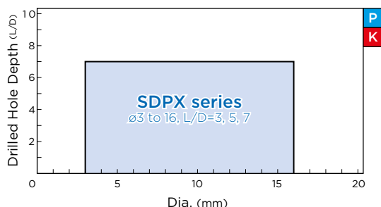
High-efficiency MULTIDRILL SDPX series
