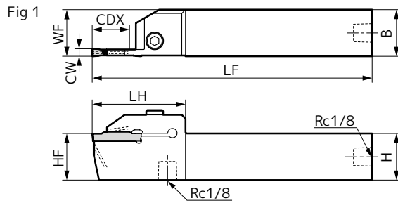
Figure shows right-handed (R) tool.
