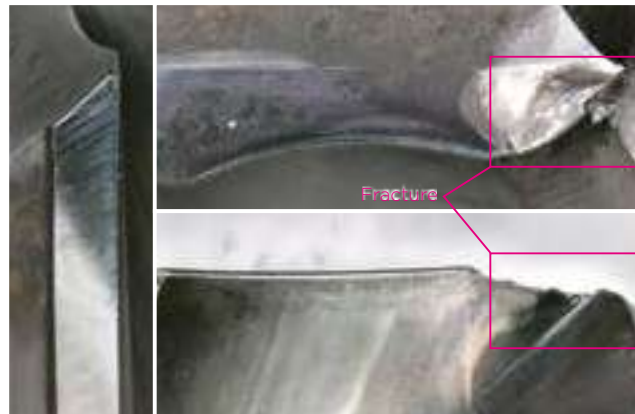
After drilling 1,000 workpieces (5 holes per workpiece)
