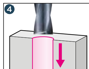
Interrupted drilling
