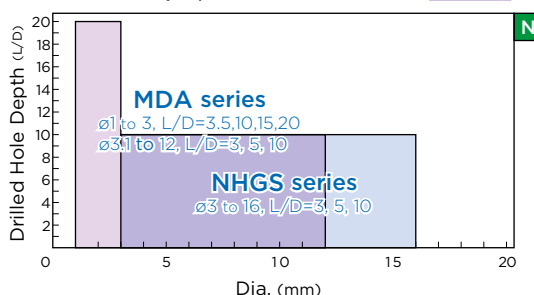
Aluminum Alloy Super MULTIDRILL NHGS series
