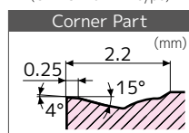
Chipbreaker Cross Section (CNMG120400 type)
