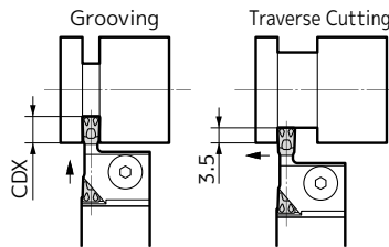
Effective Machining Depth
