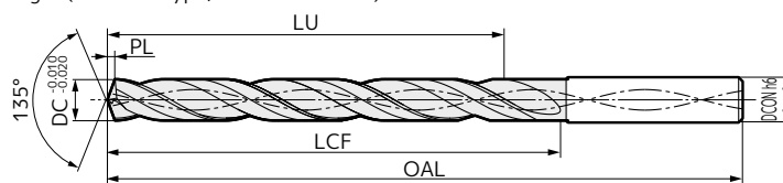
Fig 2 (NHGS10 type, ø3.0 to 16.0mm)
