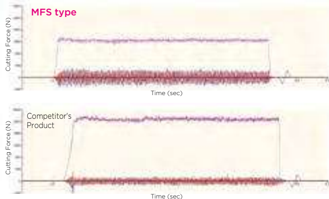
Comparison of Cutting Force
