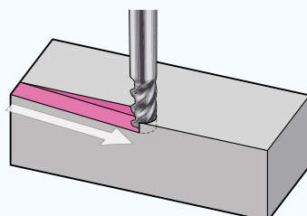
(4) Ramping GSXVL series ◎ / GSV series ○
