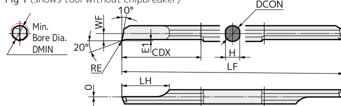
Fig 1 (shows tool without chipbreaker)
