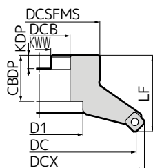
(Shell type Example)
