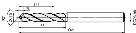
Fig 1 (Diameter ø2.0 to 4.0mm)
