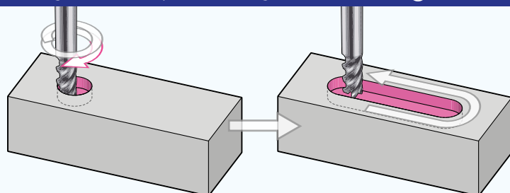
(7) Helical Milling to Groove Expansion Milling x 2 GSXVL series ◎ / GSV series ◎
