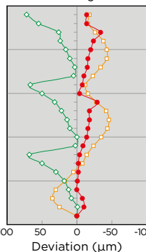
Shoulder Milling Precision
