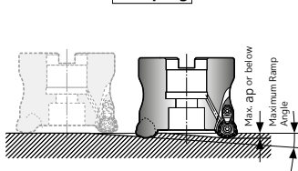
Ramping
