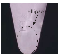
Elliptical Cutting Edge Shape
