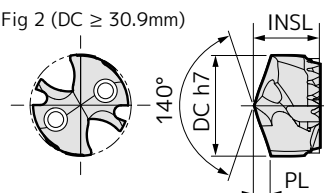
Indexable Head MTL type Diameter ø28.2 to 42.5mm
