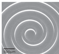
Example of Cutting Using a Nano Endmill
