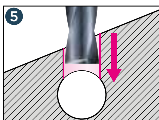
Cross drilling
