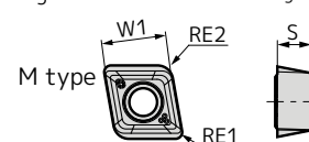
Fig 4 For stainless steel drilling
