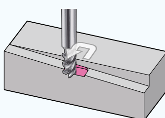
(5) Seat Face Expansion Milling GSXVL series ◎ / GSV series ◎
