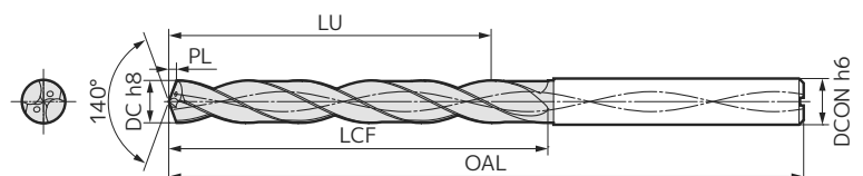
(Drill Example)
