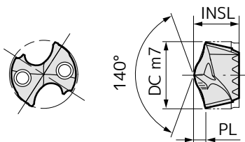
Indexable Head MEL type Diameter ø28.2 to 30.8mm
