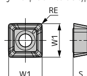
Fig 2 Peripheral insert G type
