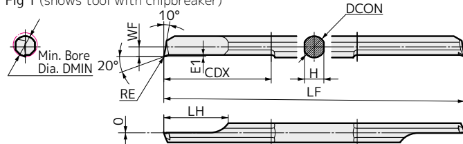
Fig 1 (shows tool with chipbreaker)
