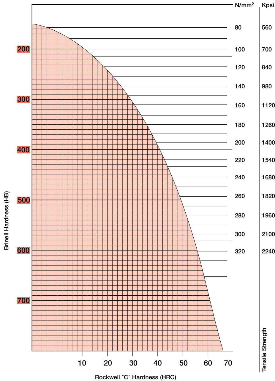
Hardness Conversion Table
