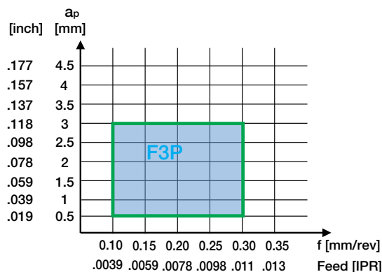
DCMT 13T504-F3P-SL Application Range
