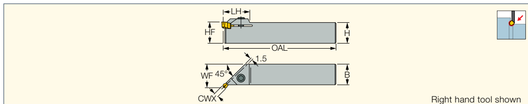
Right hand tool shown
