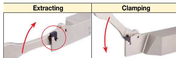
ETG 3-4 (for 3 and 4 mm, .118" and .157" tools)
