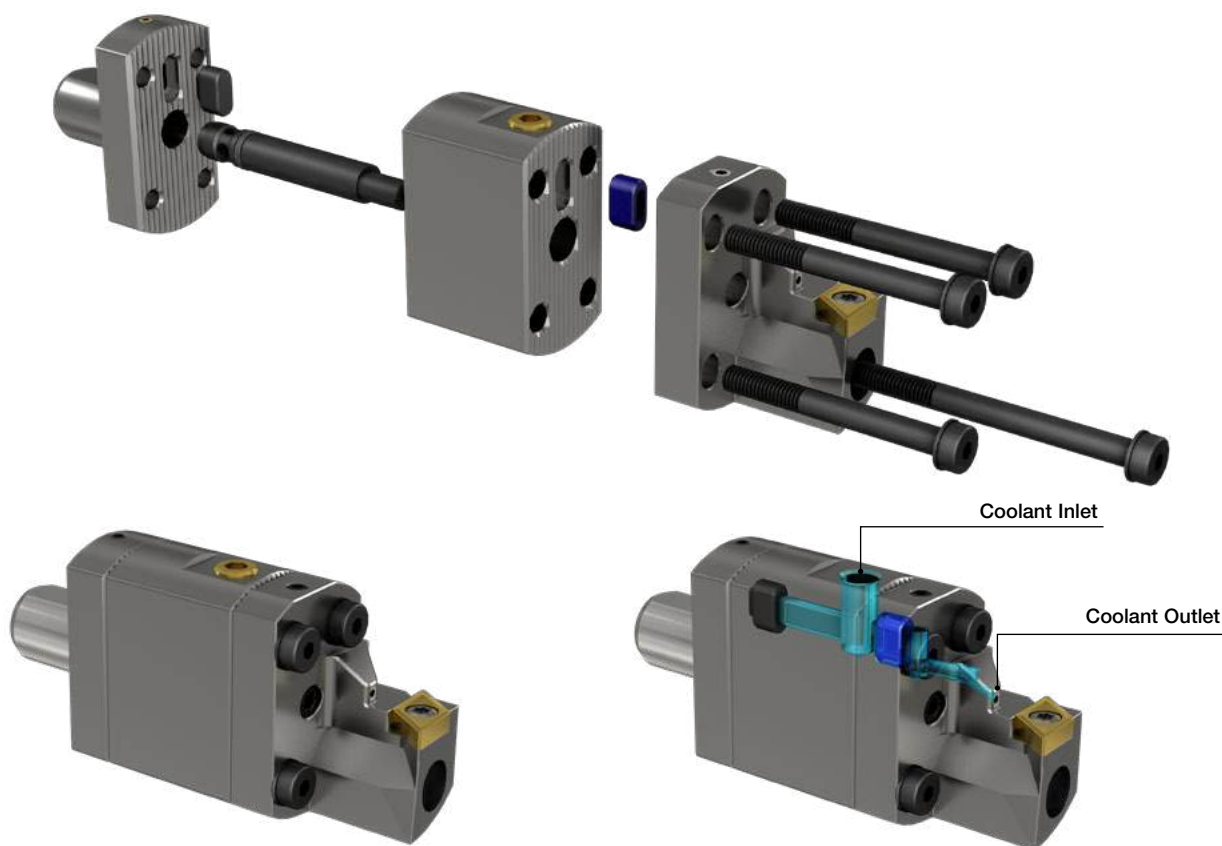
SBTB1620SRWD + SBTS30S-JHP + SBTT-SDJCR11-JHP
