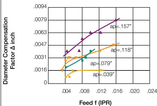
Insert: GIP 6.00E-0.8 Toolholder: GHDR 25-5
