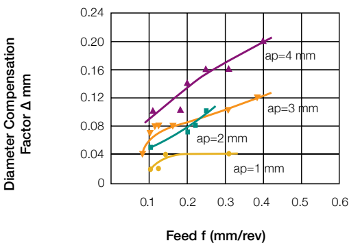
Insert: GIP 6.00E-0.8 Toolholder: GHDR 25-5
