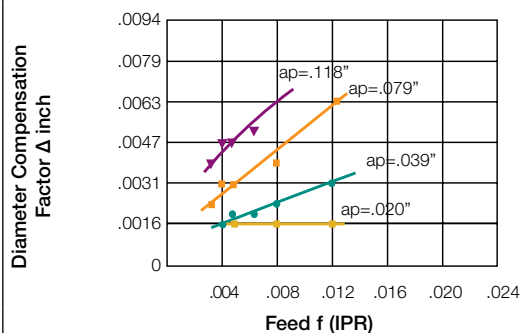
Insert: GIP 6.00E-0.8 Toolholder: GHDR 25-5
