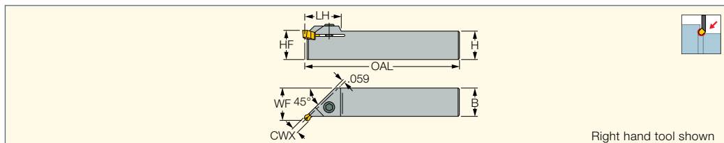
Right hand tool shown
