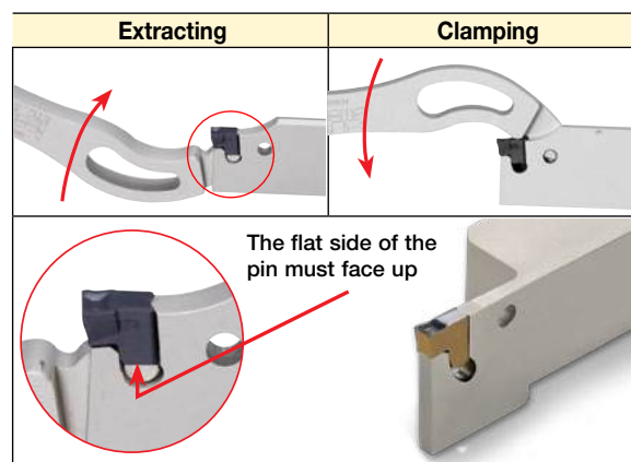
ETG 5-7 (for 5-7 mm, .197-.276" tools)
