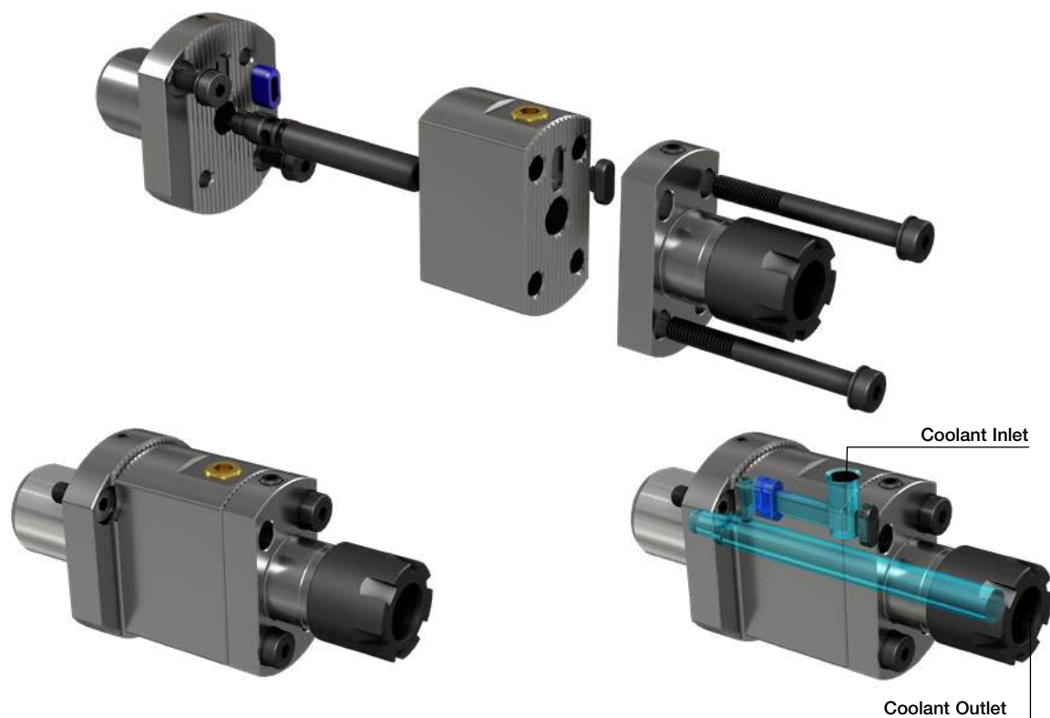
SBTB2225SRWD + SBTS30S-JHP + SBTH-ER16
