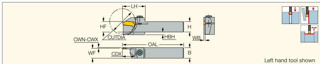
Left hand tool shown
