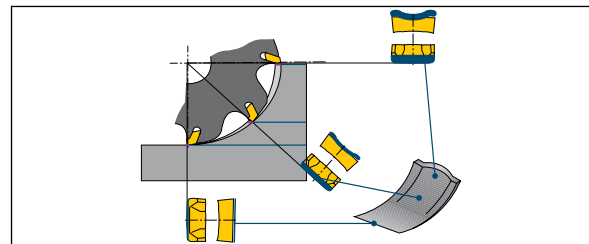
Chip Thickness as a Function of D.O.C. to Diameter Ratio
