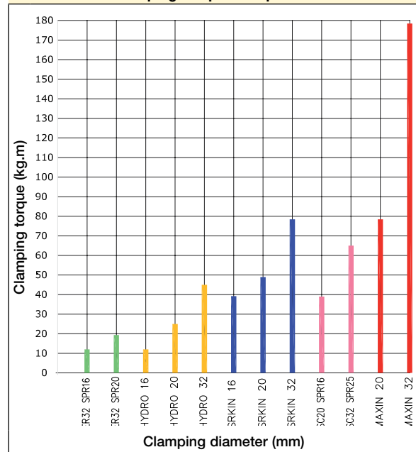
Clamping Torque Comparison
