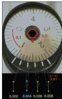
Graduated dial of 0.01 mm with circular vernier of 0.002 mm
