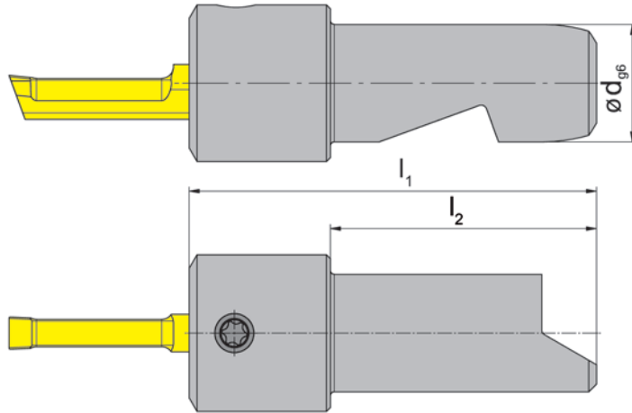
Abbildung = System SB105
