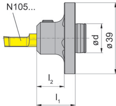
Abbildung = System SB105
