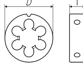
TYPE:2 D \geq 63
