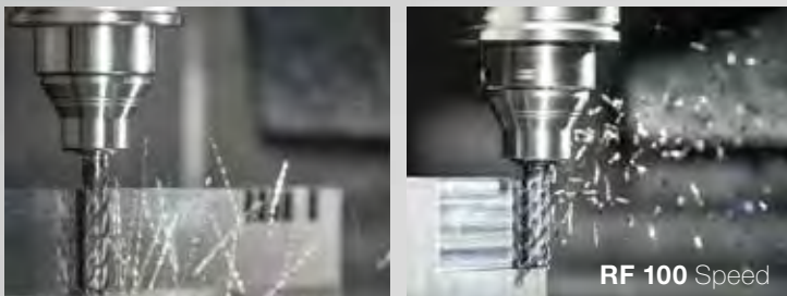
Chip formation using a conventional end mill (left) versus the RF 100 Speed (right).
