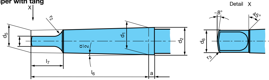
Form B, Morse taper with tang
