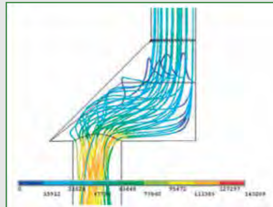
Flow conditions in the coolant duct connection slot at the point of the tapered transition
