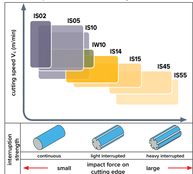
Grade and Speed Recommendation Gray Cast Iron -Finish
