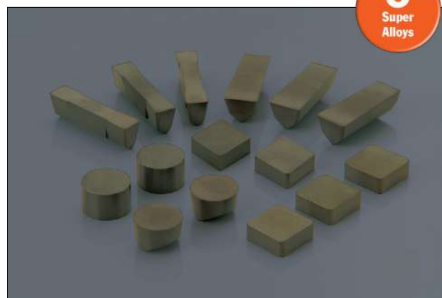
SiAlON ceramics for roughing heat resistant super alloys with scale.
