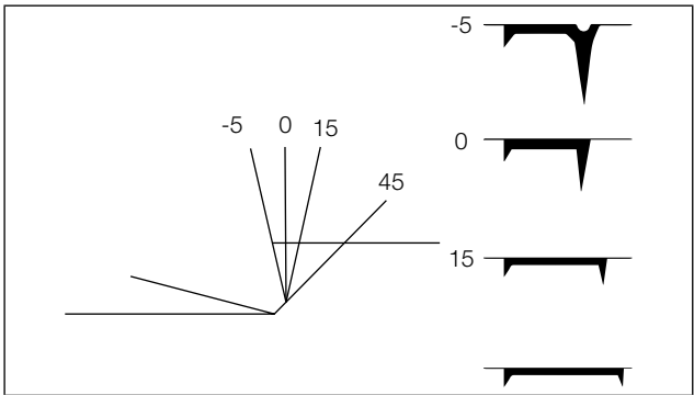
Effect of lead angle on wear pattern
