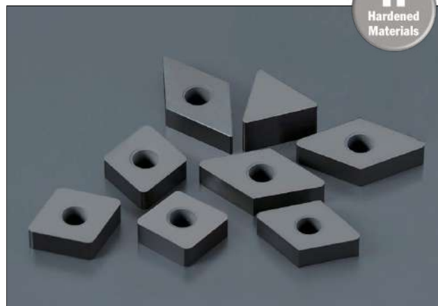
For continuous machining of hardened materials. Alumina TiC-based Ceramics.
