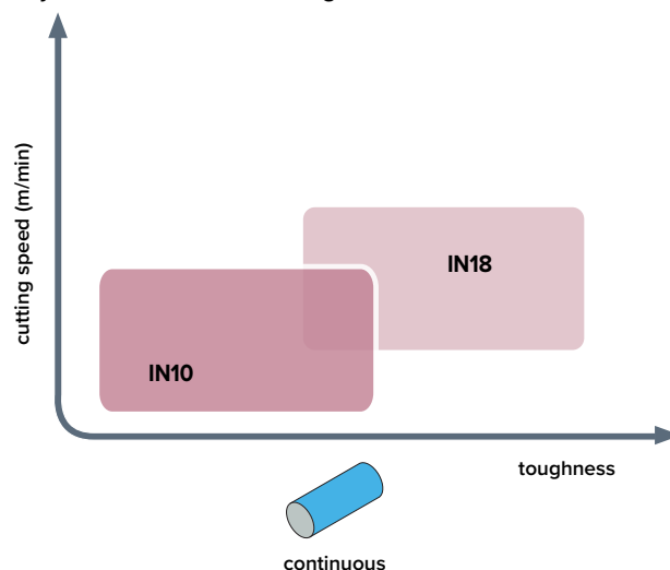
Grade and Speed Recommendation Chart Gray Cast Iron - Finish Turning
