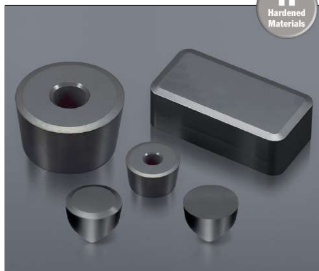
For continuous machining of gray cast iron and hardened materials Alumina TiC-based ceramics.
